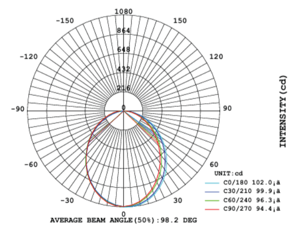
LUMINOUS INTENSITY DISTRIBUTION
